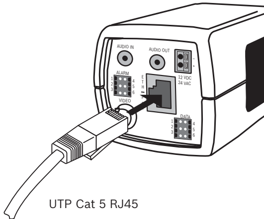
Figure 5.1 Network connection
