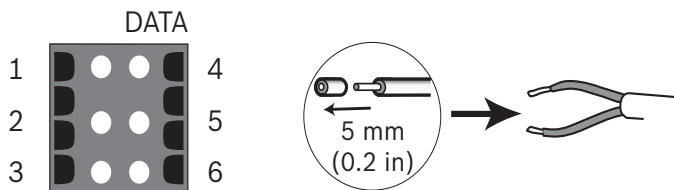
Figure 5.6 Data connector pins
