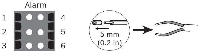
Figure 5.3 Alarm and relay connector pins
