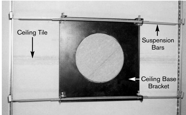
Photo 2: Ceiling Mounting (Top View)
