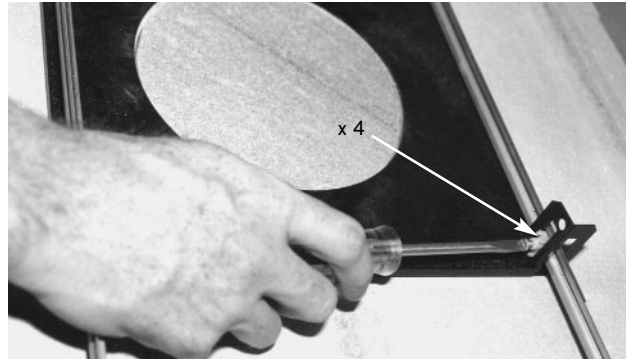
Photo 4: Bracket Securing Screws
