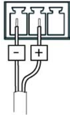
DC power input 24-34 V DC, max 17.1 W
