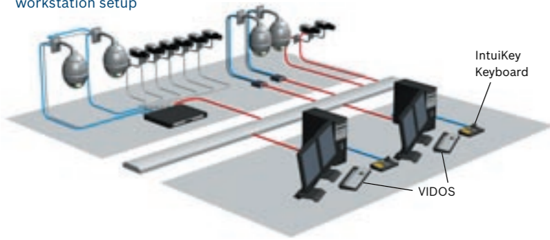
VIDOS Pro Suite - Basic stand-alone workstation setup
